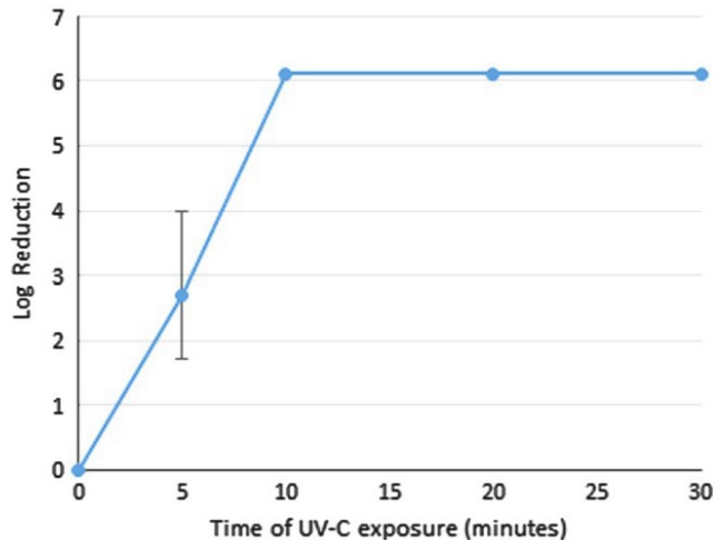
FIGURE 1. Log reduction of MHV-A59 following Surfaced UV-C exposure at a 4-foot distance (1.22 m). Virus was reduced by 2.71 log 10 in 5 minutes and by 6.11 log 10 in 10 minutes to undetectable levels. Results are the means of triplicate samples.
